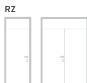
RZ Ceiling-height frame with cross rail but without transom, with top panel up to a clear frame height of 2,520 mm (single leaf, double leaf)
