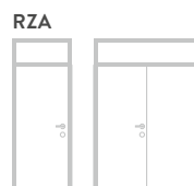
RZA Ceiling height frame with crossbar, transom and fanlight up to a clear frame height of 2,520 mm (single leaf, double leaf)
