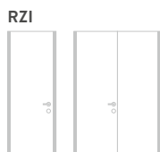
RZI Ceiling-height frame without cross rail and transom up to a clear ceiling height of 2,600 mm (single leaf, double leaf)
