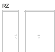
RZ Ceiling-height frame with cross rail but without transom up to a clear frame height of 2,520 mm (single leaf, double leaf)
