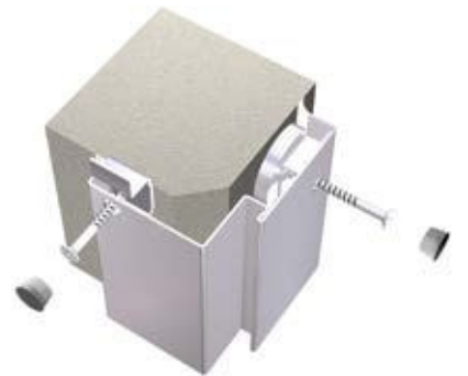
STEEL CASING 24 PROFILE Corner casing Retrofit (renovation)
