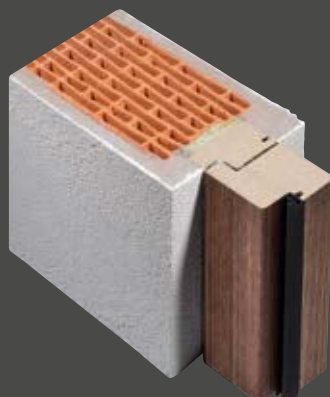
RST FRAME fitted in the embrasure with subframe
