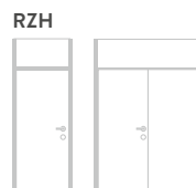
RZH Ceiling-height frame without cross rail, with transom and fanlight up to a ceiling height of 2,600 mm (single leaf, double leaf)
